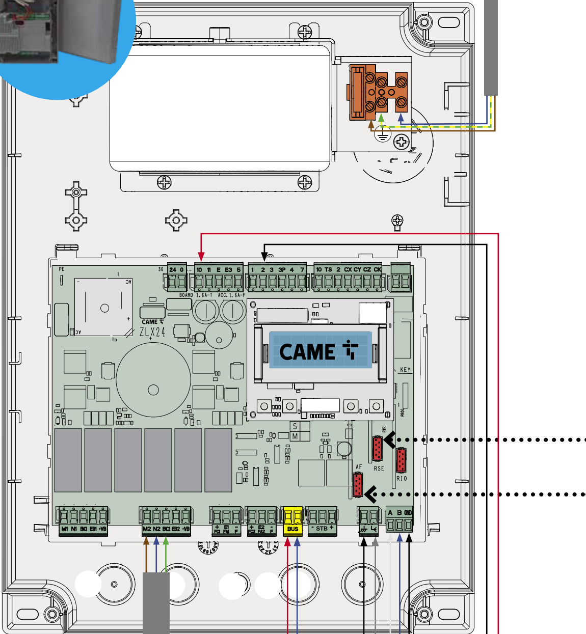
RSE Set RSE jumper to OFF
