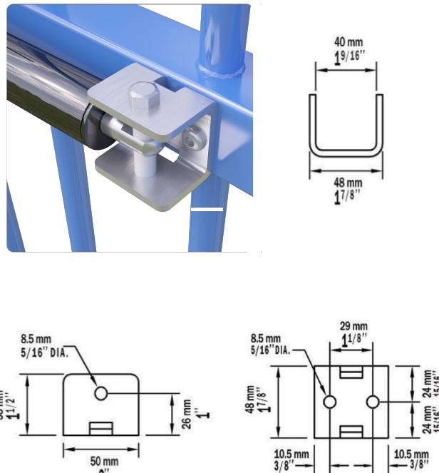
Gate Bracket
