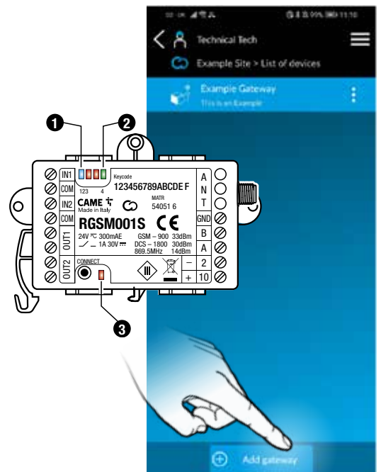
3.9 The RED 3 and GREEN 2 LED's will now be on solid and the BLUE 1 flashing 1x/sec. CONGRATULATIONS - the RGSM001S has now been successfully added to the Connect platform
