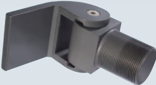
SureClose SM AT90 W Code: 75108114 NON-SELF-CLOSING • Gate sweep: 180° one way
