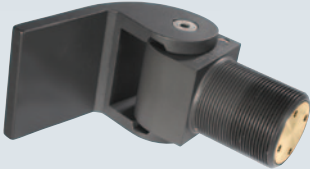
SureClose 57 AT90 W Code: 75057214m SELF-CLOSING FROM 85° • Gate sweep: 180° one way • Holds gate open at 90°–180° (not suitable for pool/safety gates) • Adjustment tool included
