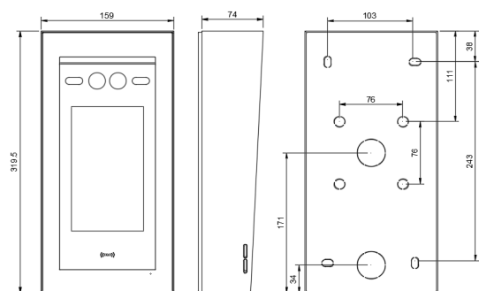
Surface-mount
