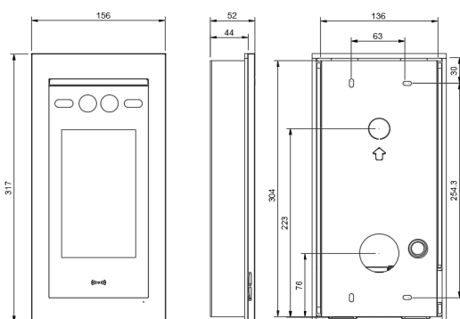
Flush-mount
